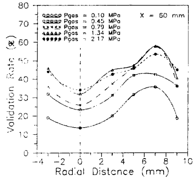
Fig. 5 Validation rate for different radial positions and ambient gas pressure
