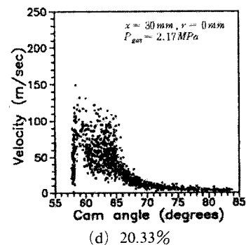
Fig. 8 Comparison of velocity only and velocity data obtained when both velocity and diameter data were acquired. Measurement position and condition: x=30 mm, r=0 mm, P_{gas}=0.1 MPa and 2.17 MPa
