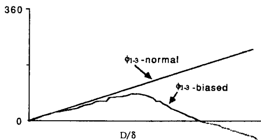
Fig. 3 Schematic of the instrument response curve for the normal and biased case
