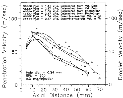
Fig. 7 Penetration velocity and droplet velocity at the spray tip for different ambient gas pressure, determined from high-speed photograph, and the measured velocity data
